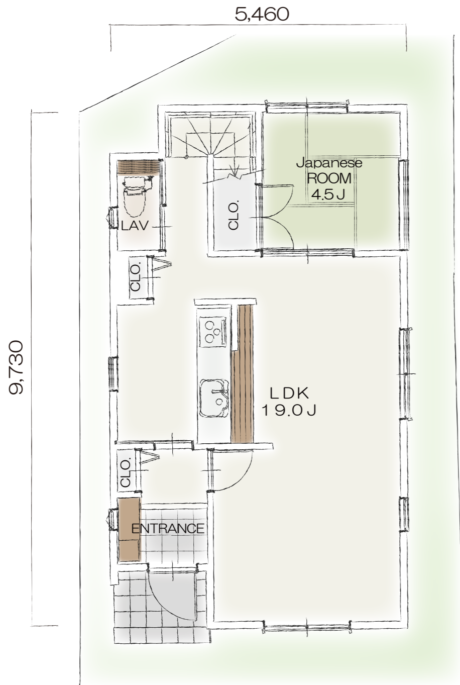
1F PLAN
