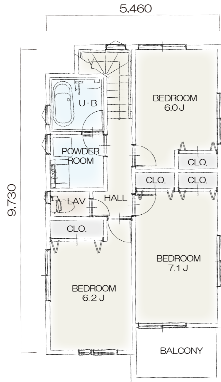
2F PLAN
