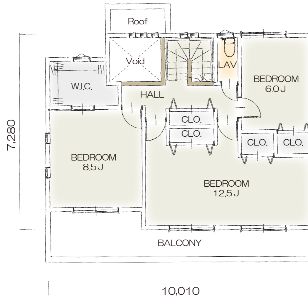
2F PLAN
