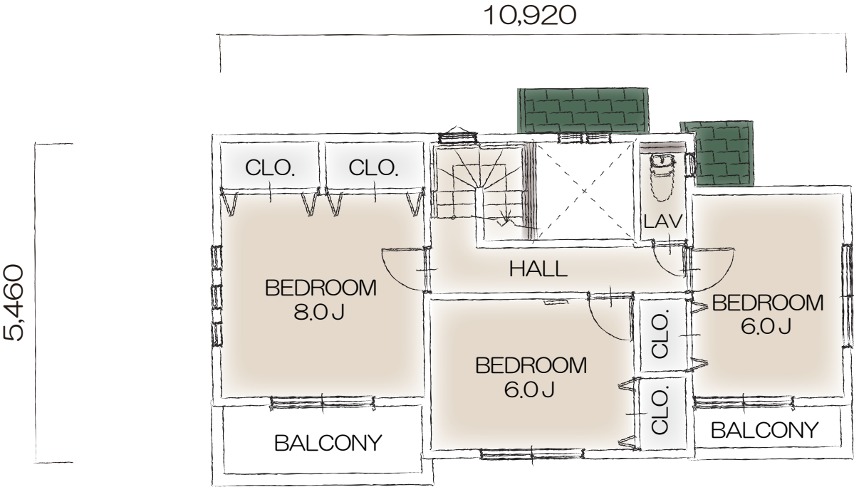
2F PLAN
