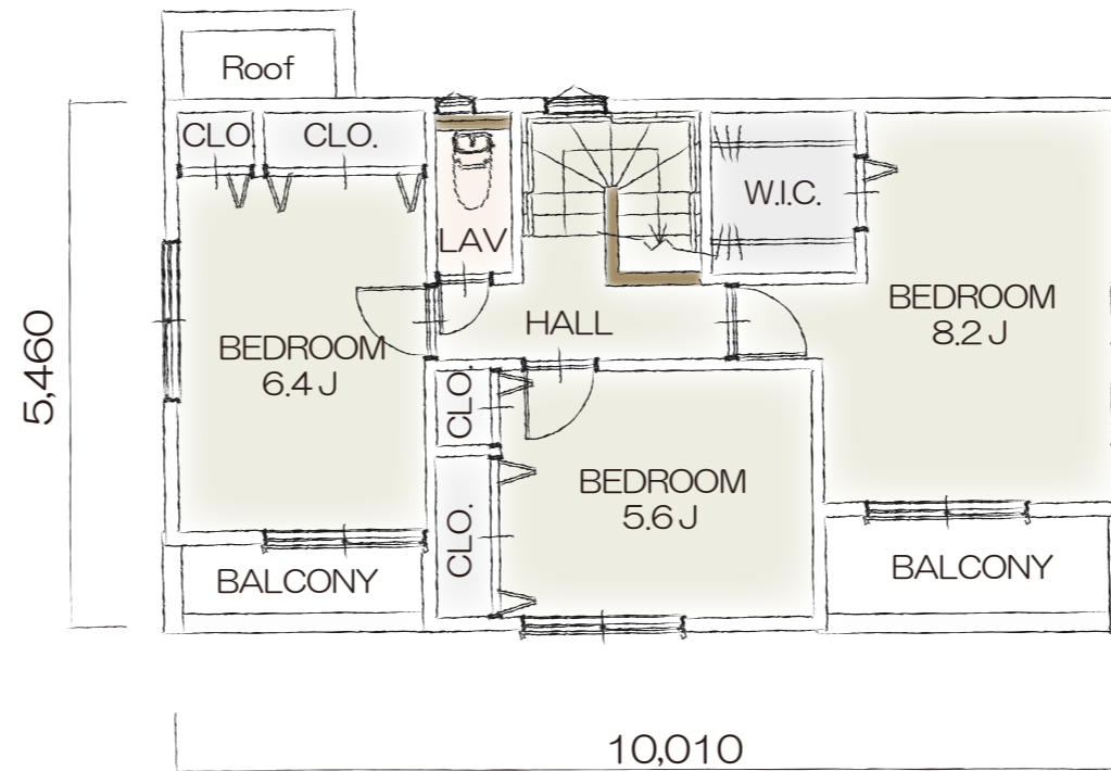
2F PLAN
