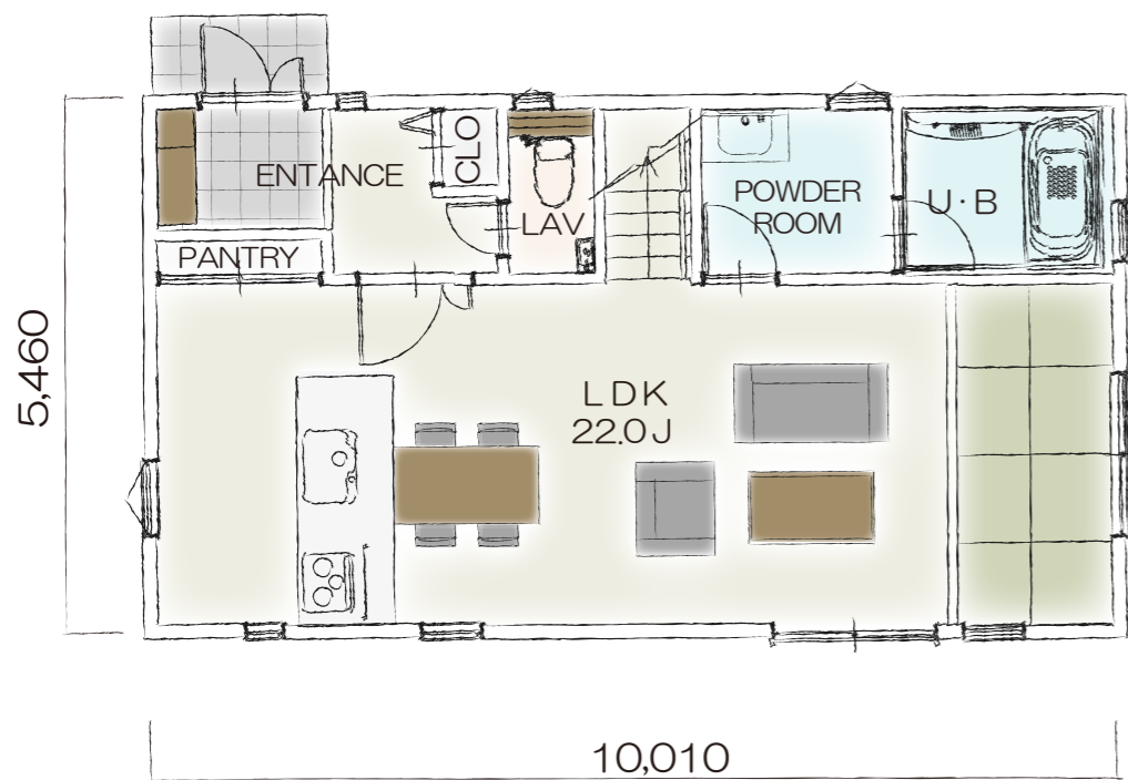
1F PLAN
