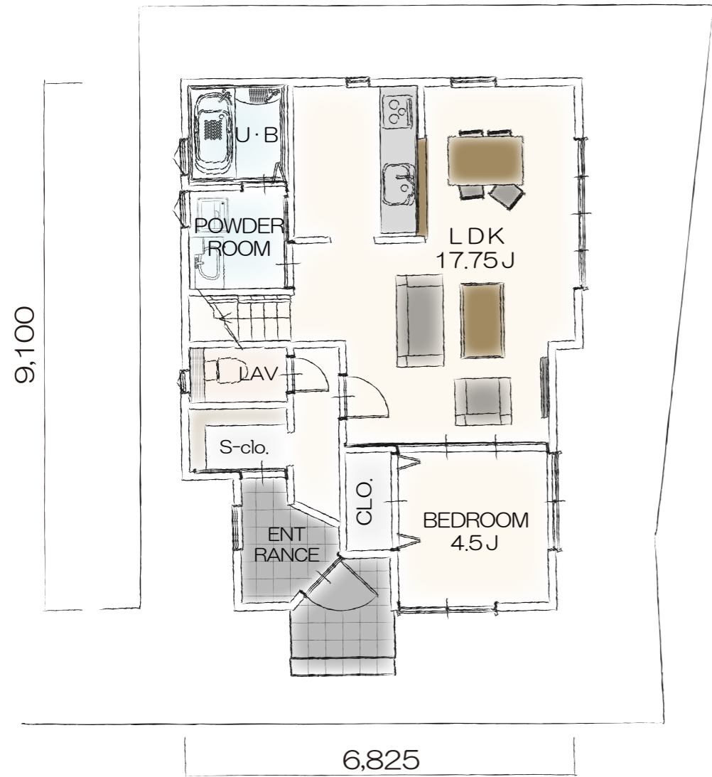
1F PLAN
