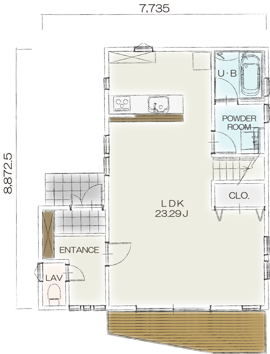
1F PLAN
