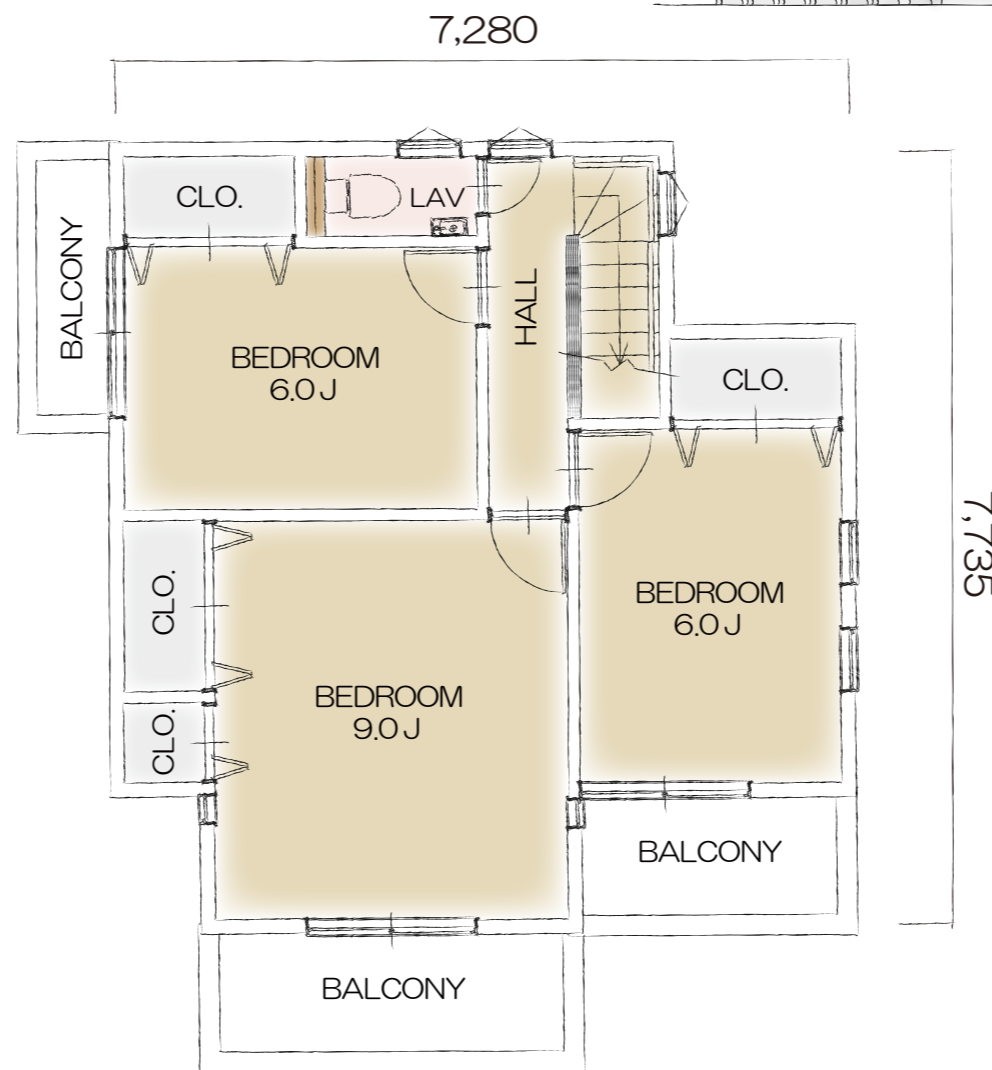
2F PLAN
