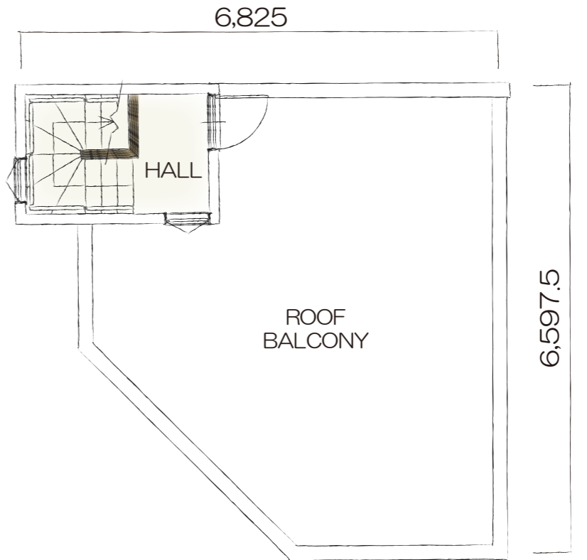
PHF PLAN
