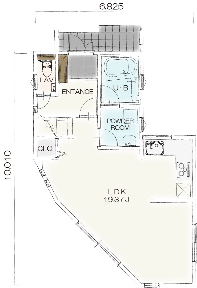
1F PLAN
