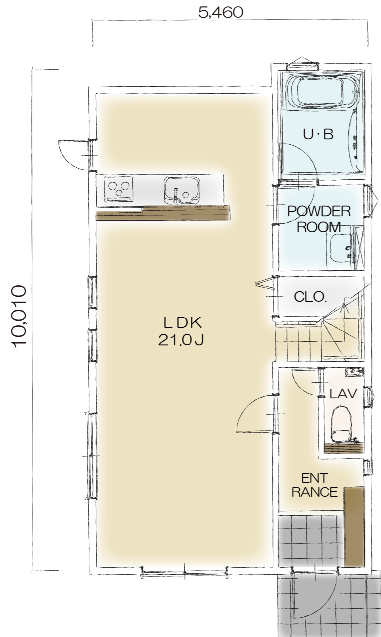
1F PLAN
