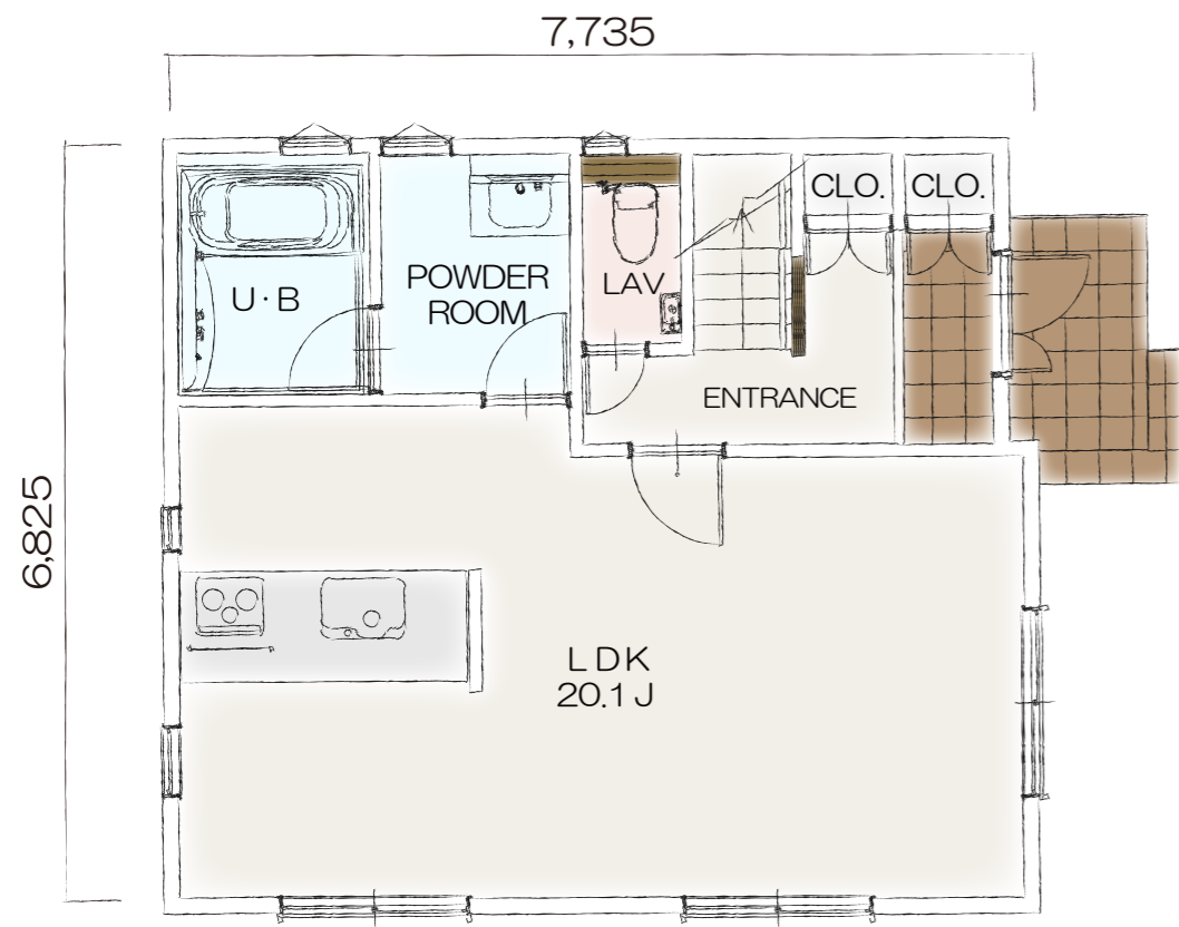
1F PLAN
