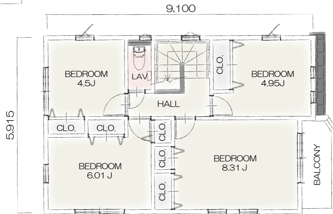
2F PLAN
