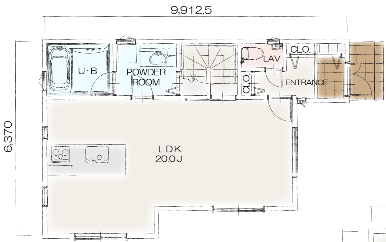
1F PLAN
