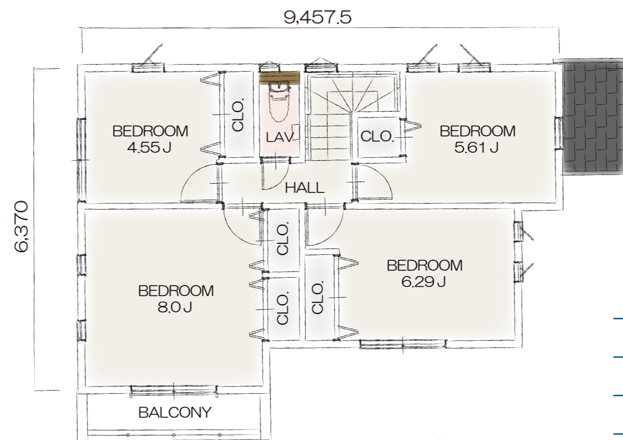
2F PLAN
