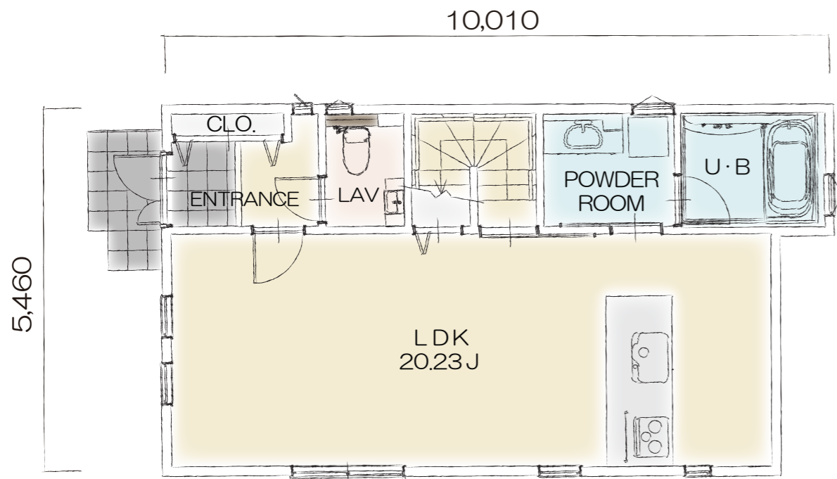
1F PLAN
