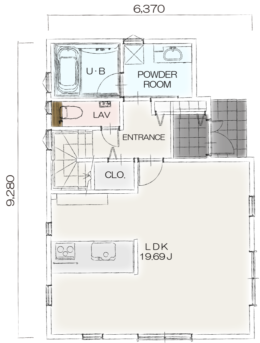
1F PLAN
