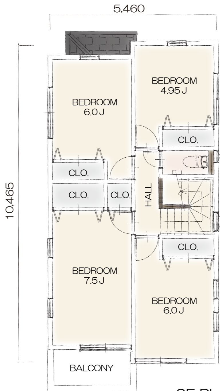
2F PLAN
