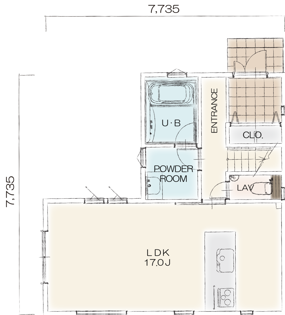
1F PLAN
